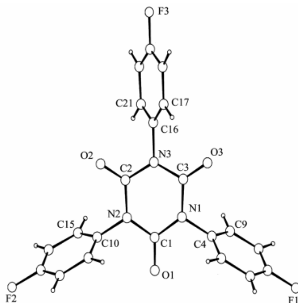
Figure 1. A perspective view and labelling scheme for molecule 4 ; selected bond lengths [Å] and angles [°]: N(1)–C(1) 1.379(3), N(1)–C(3) 1.398(3), N(1)–C(4) 1.454(3), N(2)–C(1) 1.384(3), N(2)–C(2) 1.386(3), N(2)–C(10) 1.452(3), N(3)–C(2) 1.382(3), N(3)–C(3) 1.391(3), N(3)–C(16) 1.454(3), O(1)–C(1) 1.212(3), O(2)–C(2) 1.204(3), O(3)–C(3) 1.197(3), C(1)–N(1)–C(3) 124.8(2), C(1)–N(2)–C(2) 124.3(2), C(2)–N(3)–C(3) 124.8(2), N(1)–C(1)–N(2) 115.6(2), N(2)–C(2)–N(3) 115.7(2), N(1)–C(3)–N(3) 114.5(2); the central 6-membered ring of compound 4 N(1)–N(2)–N(3)–C(1)–C(2)–C(3) is planar, deviations from the least-squares plane do not exceed 0.027 Å; the C(4)–C(9), C(10)–C(15), and C(16)–C(17) benzene rings are twisted out of this plane by 66.5, 66.7, and 65.3°; the main bond lengths and angles in 4 are virtually the same as in the previously studied [9] C 3 N 3 O 3 (C 6 H 5 ) 3
