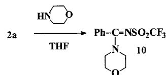
Scheme 15. Synthesis of substitution product 10
