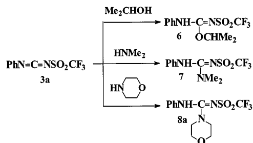
Scheme 11. Reactions between carbodiimide 3a and alcohols and secondary amines
