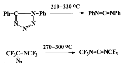
Scheme 3. High-temperature reactions
