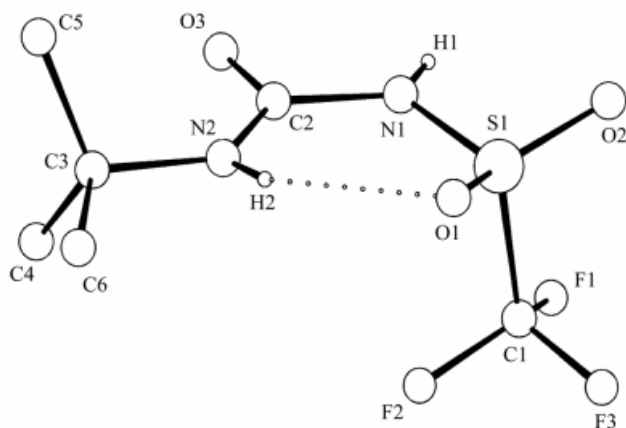
Figure 2. A perspective view and labelling scheme for molecule 5 ; selected bond lengths [Å] and angles [°]: S(1)–O(1) 1.413(2), S(1)–O(2) 1.409(2), S(1)–N(1) 1.596(2), S(1)–C(1) 1.809(3), O(3)–C(2) 1.225(2), N(1)–C(2) 1.421(3), N(2)–C(2) 1.310(3), N(2)–C(3) 1.485(2), O(1)–N(2) 2.837(3); O(1)–H(2)–N(2) 142(3), S(1)–N(1)–C(2)–O(3) –168.2, N(1)–C(2)–N(2)–C(3) 178.3, O(3)–C(2)–N(2)–C(3) –1.7
