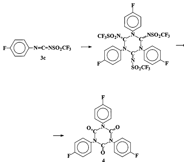
Scheme 8. Formation of triazinetrione 4
