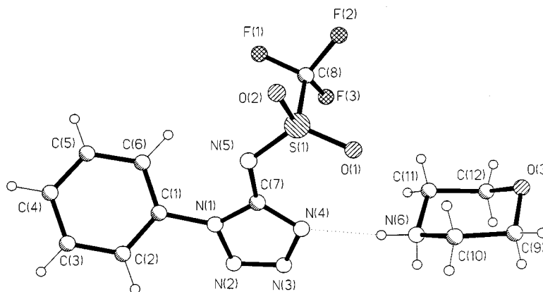
Figure 3. A perspective view and labelling scheme for molecule 9 ; selected bond lengths [Å] and angles [°]: S(1)–O(1) 1.419(2), S(1)–O(2) 1.431(2), S(1)–N(5) 1.531(3), S(1)–C(8) 1.806(4), N(1)–C(7) 1.355(4), N(1)–N(2) 1.356(4), N(1)–C(1) 1.427(4), N(2)–N(3) 1.284(4), N(3)–N(4) 1.351(4), N(4)–C(7) 1.330(4), N(5)–C(7) 1.351(4); N(2)–N(1)–C(7) 108.5(2), N(1)–N(2)–N(3) 105.9(3), N(2)–N(3)–N(4) 112.1(2), N(3)–N(4)–C(7) 105.9(3), N(1)–C(7)–N(4) 107.5(3), S(1)–N(5)–C(7) 123.5(2)
