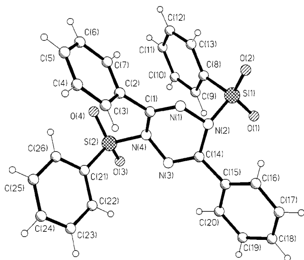
Figure 4. A perspective view and labelling scheme for molecule 12 ; selected bond lengths [Å] and angles [°]: S(1)–N(2) 1.667(5), S(1)–C(8) 1.763(7), S(2)–N(4) 1.708(5), S(2)–C(21) 1.749(7), N(1)–C(1) 1.269(7), N(1)–N(2) 1.458(6), N(2)–C(14) 1.416(7), N(3)–C(14) 1.271(7), N(3)–N(4) 1.411(6), N(4)–C(1) 1.409(7); N(2)–N(1)–C(1) 113.8(5), N(1)–N(2)–C(14) 115.4(4), N(4)–N(3)–C(14) 114.4(4), N(3)–N(4)–C(1) 116.5(4), N(1)–C(1)–N(4) 121.0(5), N(2)–C(14)–N(3) 120.9(5)
