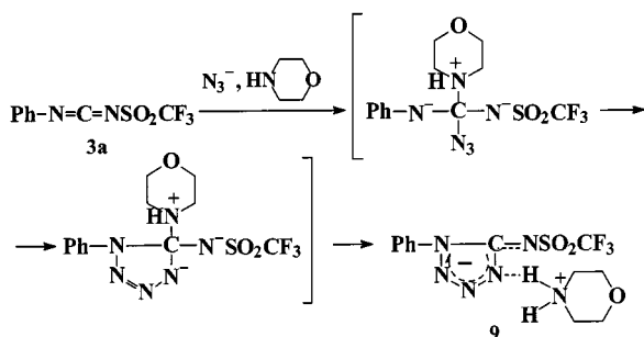
Scheme 14. Formation of morpholinium salt 9
